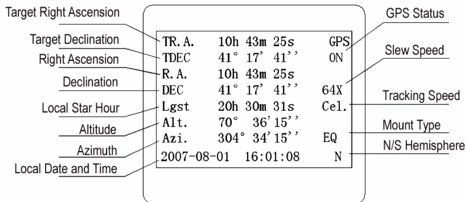
Figure 17. 8401 HC LCD Information Screen
