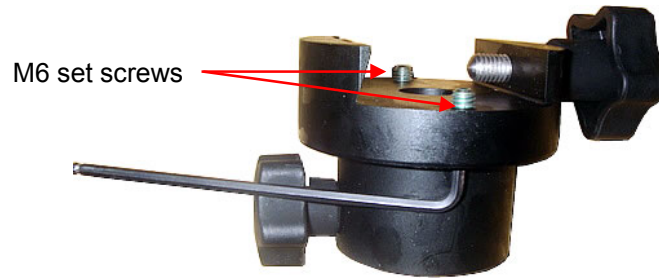
Figure 14. Secondary dovetail and set screws
