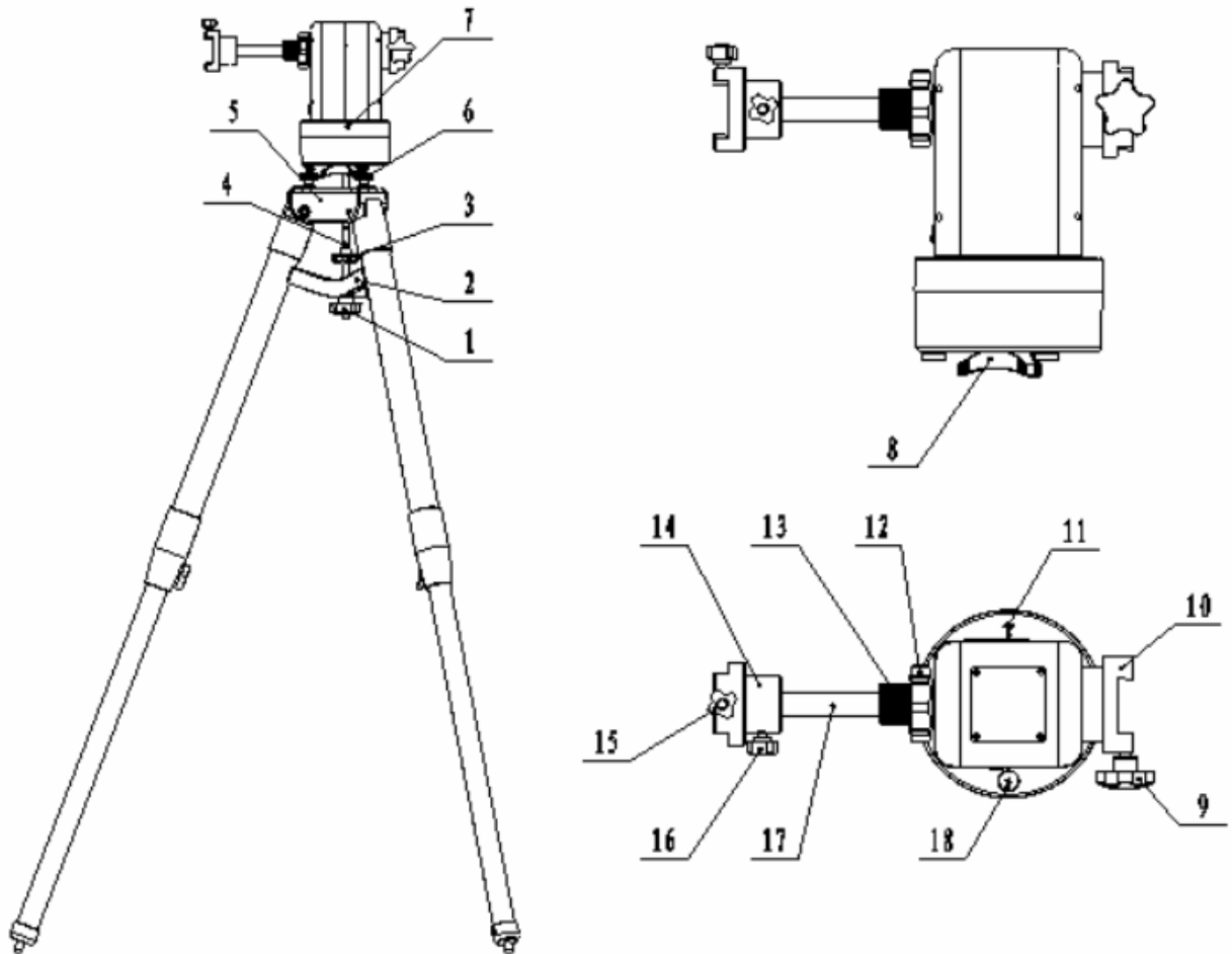
Figure 3. MT2 assembly term
